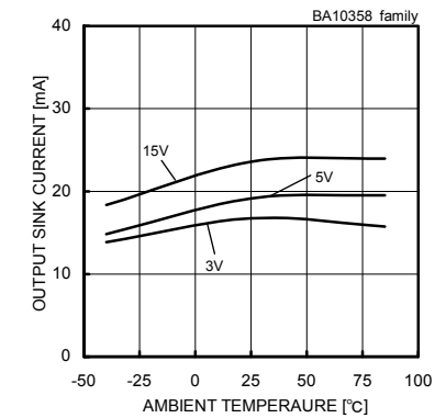
Fig. 9 Output Sink Current - Ambient Temperature (VOUT=VCC)
