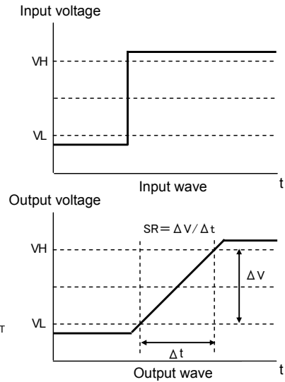
Fig. 122 Slew Rate Input Waveform
