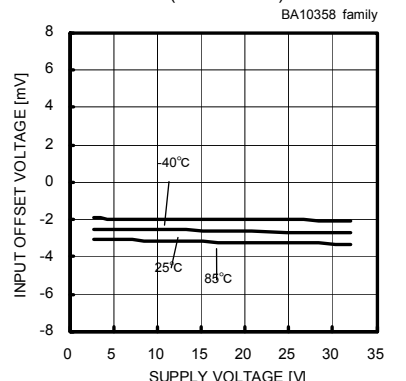
Fig. 12 Input Offset Voltage - Supply Voltage (Vcm=0[V], VOUT=1.4[V])
