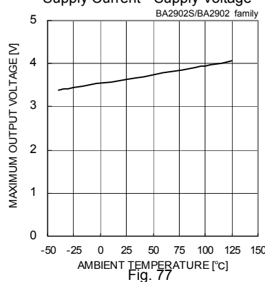
Fig. 77 Maximum Output Voltage - Ambient Temperature(VCC=5[V],RL=2[kΩ])
