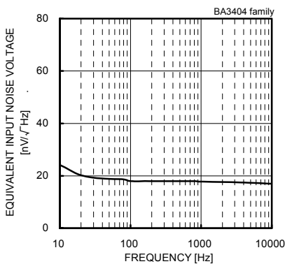
Fig. 118 Equivalent Input Noise Voltage - Frequency (VCC/VEE=+15[V]/-15[V], Rs=100[Ω], Ta=25[°C])
