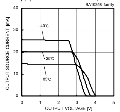
Fig. 6 Output Source Current - Output Voltage (VCC=5[V])
