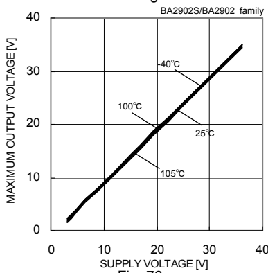
Fig. 76 Maximum Output Voltage - Supply Voltage (RL=10[kΩ])
